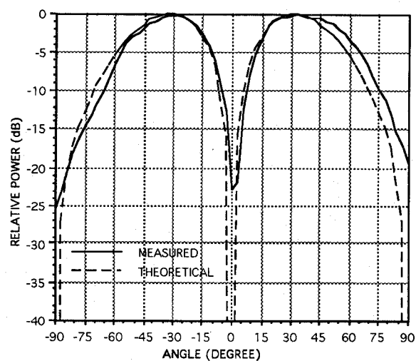
Figure 3b : Difference pattern in the azimuth plane.
