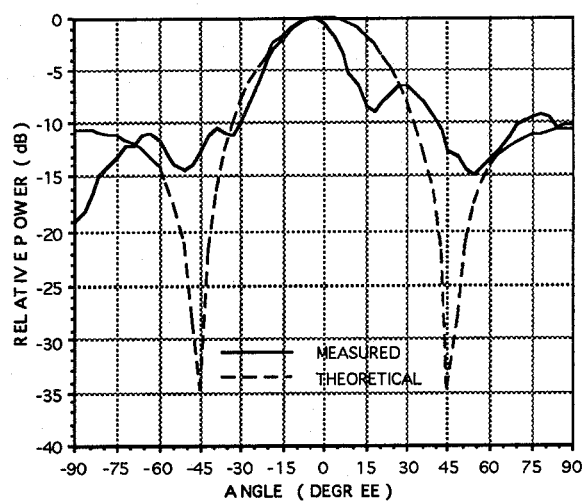
Figure 4a : Sum pattern in the elevation plane.
