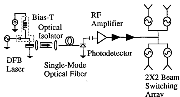
Figure 1 : System setup.
