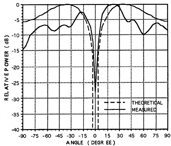
Figure 4b : Difference pattern in the elevation plane.
